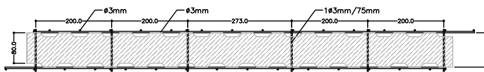
EXTERNAL MESH PANEL SIMPLE \phi 3\text{mm}
